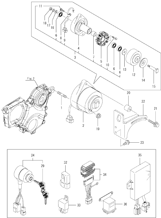
0CD11-M12701 ENGINE Fig.15. GENERATOR
