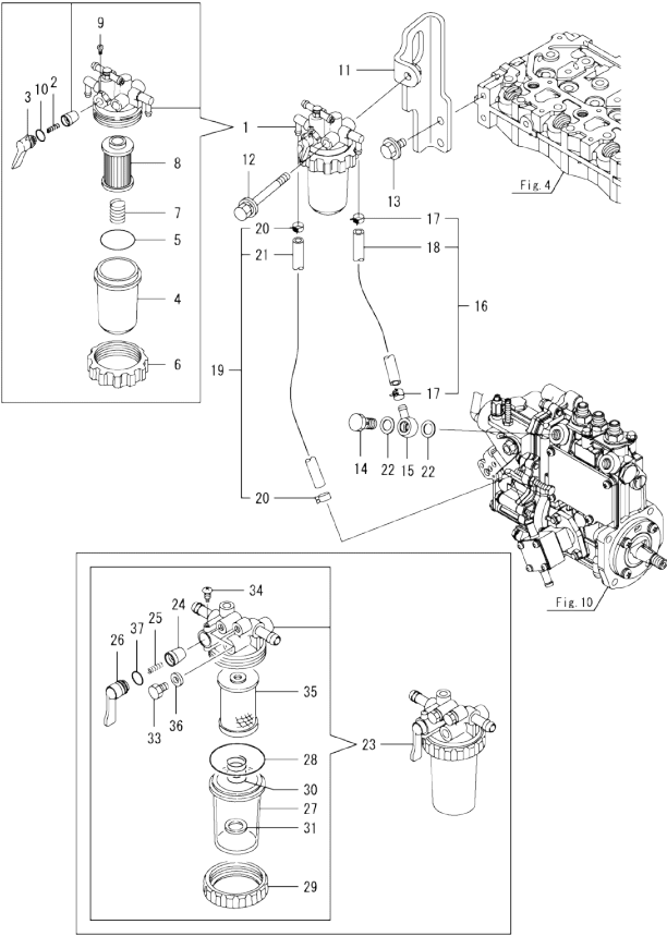
OCD11-M12701 ENGINE Fig.13. FUEL PIPE
