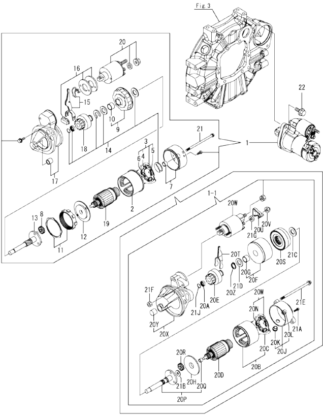
Fig.14. STARTER MOTOR
